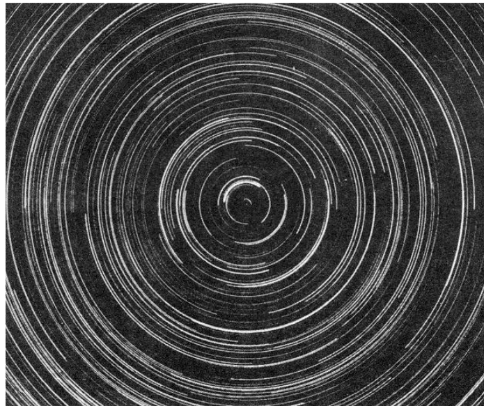
Figure 19. Time delay photo of stars and galaxies rotating around the North Pole of the celestial sphere during the night.
