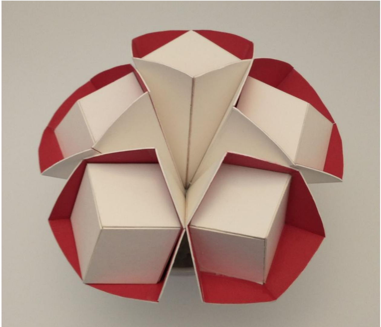
Figure 9. The sublime bouquet of the spherical-dodecahedron-singularity.
