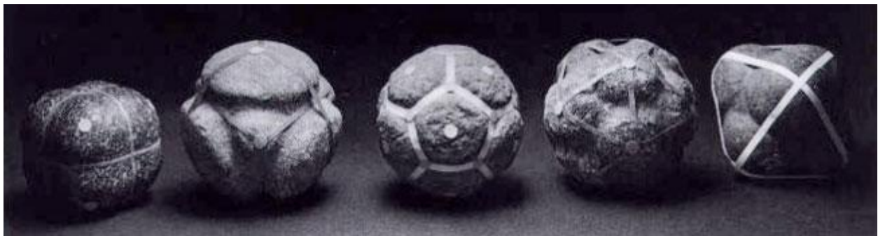
Figure 13. Spherical Cube, Octahedron, Dodecahedron, Icosahedron, Octahedron: http://www.neverendingbooks.org/the-scottish-solids-hoax
